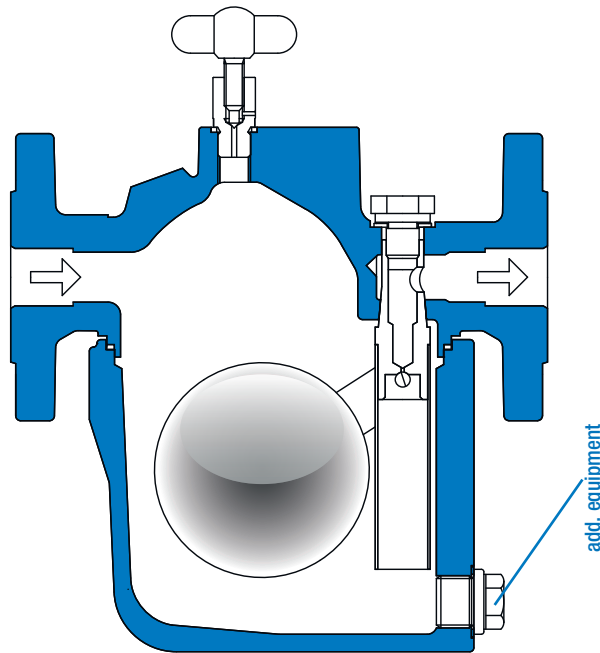
Model WU-1101 utilized as Drain Control Unit
